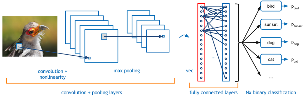
Figure 5.6: Example of a CNN used for image classification [38].
