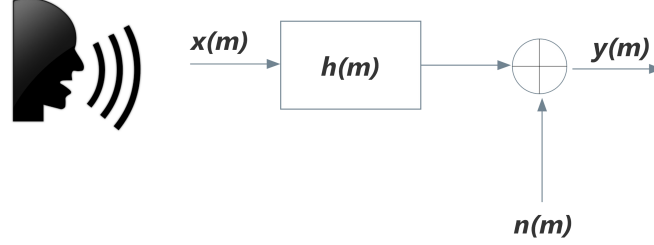
Figure 2.2: Block diagram of a speech distortion model including convolutive and additive noise as environmental distortions.
