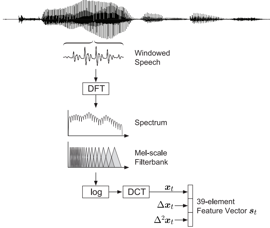
Figure 1.3: Diagram of a typical feature extractor for ASR purposes [112].
