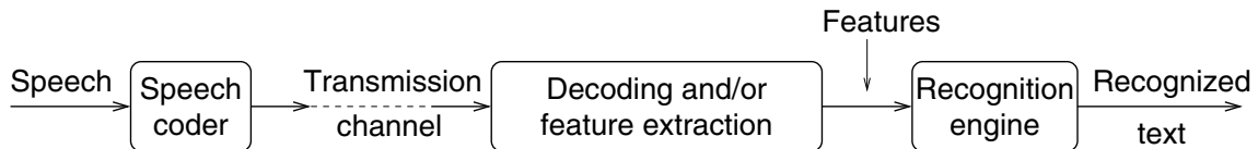
Figure 2.1: Block diagram of a network-based speech recognition scheme [149].
