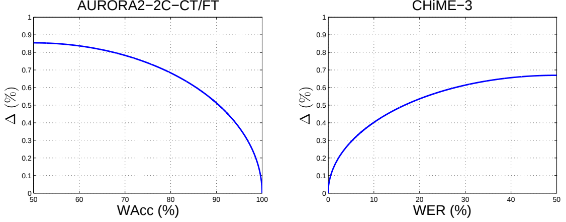
Figure 6.7: Amplitude of the 95% confidence interval as a function of WAcc for the test sets of the AURORA2-2C-CT/FT databases (left) and WER for the real data evaluation set of the CHiME-3 corpus (right).
