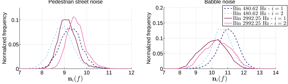
Figure 4.2: Example histograms of the variable \mathbf{n}_i(f) ( i = 1, 2 ) at two different frequency bins. These histograms are calculated for two types of noise recorded with a dual-microphone smartphone: pedestrian street (left) and babble (right) noise.
