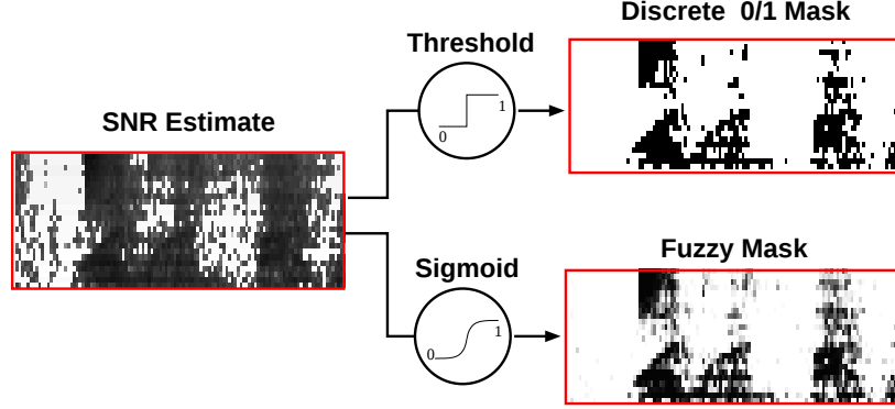
Figure 2.4: A comparison between binary and soft missing-data masks obtained from an a priori SNR estimate [14].
