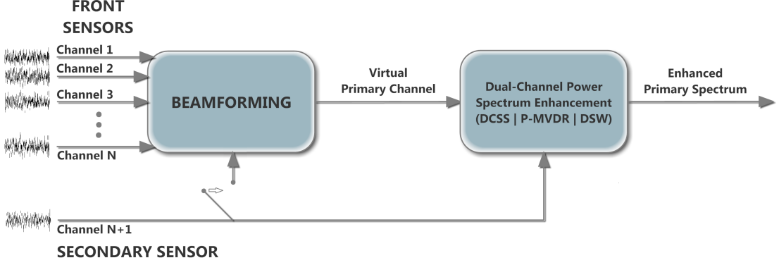
Figure 3.1: Power spectrum enhancement scheme followed when the IMD has more than one front sensor.
