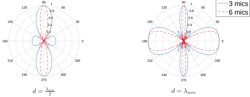
Figure 2.7: Example of spatial aliasing (right) for the microphone arrays of Figure 2.6.
